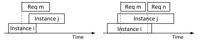
Fig. 3. Adversary situations because of the time constraint.
